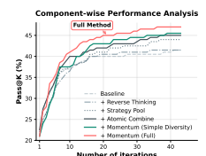
Figure 6: Component ablation shows the momentum
