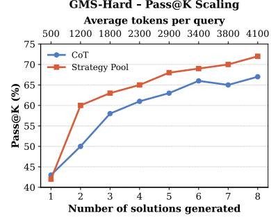
(a) GMS-Hard scaling curves.
