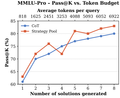
(b) MMLU-PRO scaling curves.
