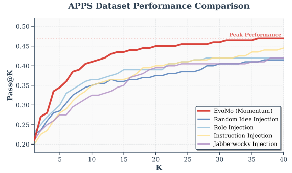
(a) Absolute performance comparison on APPS dataset
