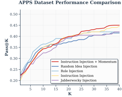
(a) Absolute performance on APPS.
