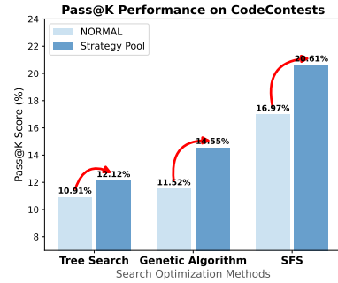
(c) CodeContests Pass@K
