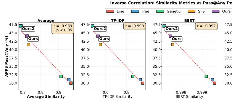
Figure 5: Diversity Analysis: Lower Similarity Correlates with Higher Pass@Any Performance in APPS dataset for 6 search method. Average denotes the per-method mean of the four similarities.
