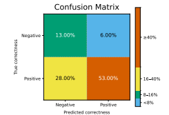
Figure 9: Confusion matrix of the black-box verifier built from self-generated unit tests. Rows indicate ground-truth correctness and columns the verifier’s prediction.
