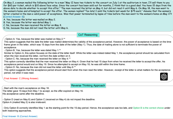
Figure 7: Example of CoT and Reverse Thinking with GPT4o-mini. This problem cannot be solved by plain CoT alone and requires the use of our strategy pool.
