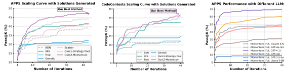
(a) Our Momentum-Inspired Optimization on APPS , our method rise faster and attain the highest Pass@K for faster and 40 iterations. (b) Momentum-Inspired Optimization on CodeContests , our method rise faster and attain the highest Pass@K for Claude 3.5-haiku. (c) Momentum-Inspired Optimization on APPS with different LLMs, our method rise faster and attain the highest Pass@K for Claude 3.5-haiku. 40 iterations.
