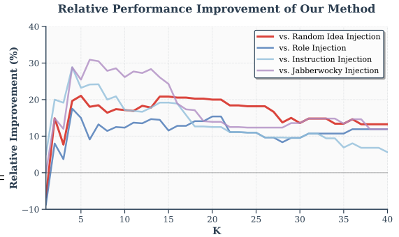
(b) Relative performance improvement over baselines
