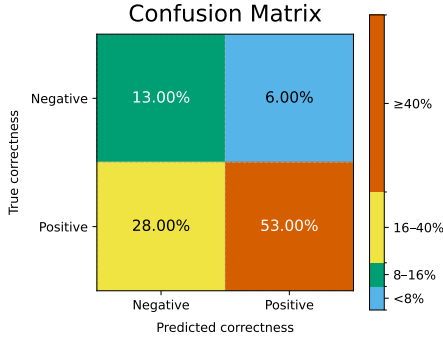
Figure 7: Confusion matrix of the black-box verifier built from self-generated unit tests. Rows indicate ground-truth correctness and columns the verifier’s prediction.
