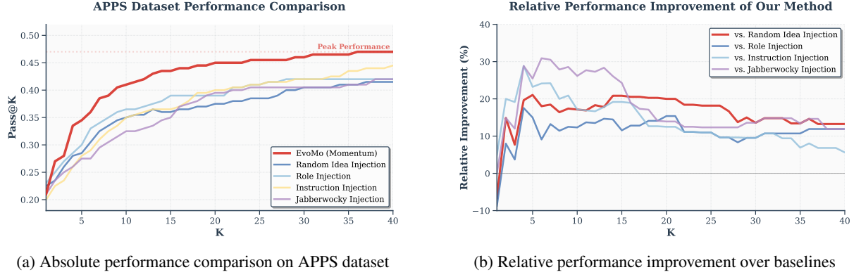
Figure 8: Performance comparison of our method EvoMo against diversified sampling baselines. (a) shows the absolute Pass@K performance across different methods, where our approach consistently outperforms all baselines. (b) illustrates the relative improvement percentage of our method over each baseline, demonstrating significant gains, especially at higher K values.
