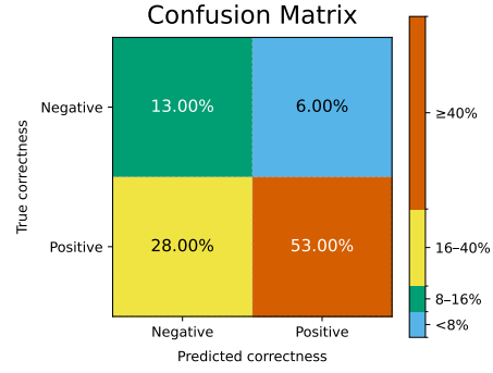
Figure 9: Confusion matrix of the black-box verifier built from self-generated unit tests. Rows indicate ground-truth correctness and columns the verifier’s prediction.
