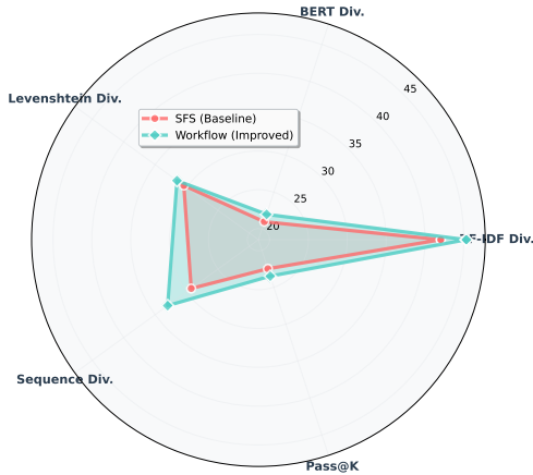
Figure 14: Workflow-augmented SFS improves diversity and accuracy. Radar plot on CODECONTESTS: higher values indicate better diversity (TF-IDF / BERT / Levenshtein / Sequence) and higher Pass@K.
