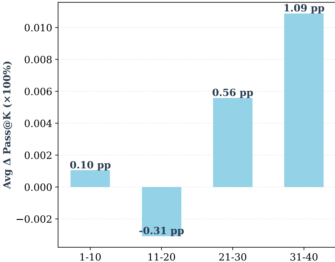
Average Gain vs Instruction by K Ranges
