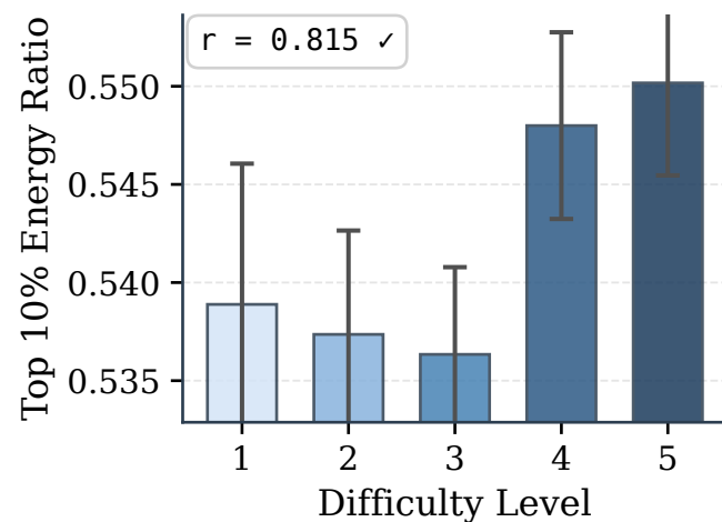
(f) Top 10% Energy Ratio - Llama 3.1 8B
