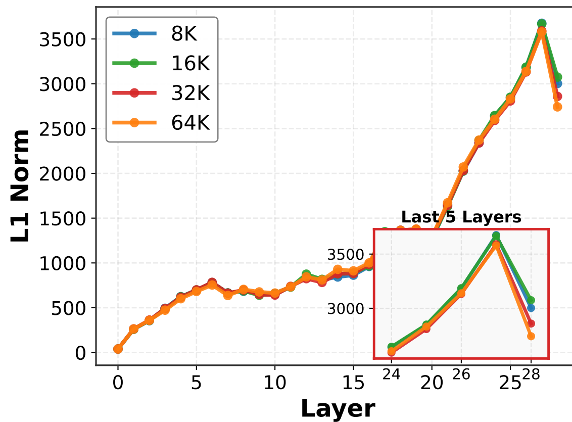
L1 Norm
