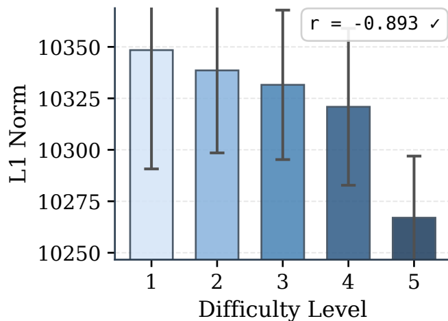
(a) L1 Norm - Qwen 2.5 7B
