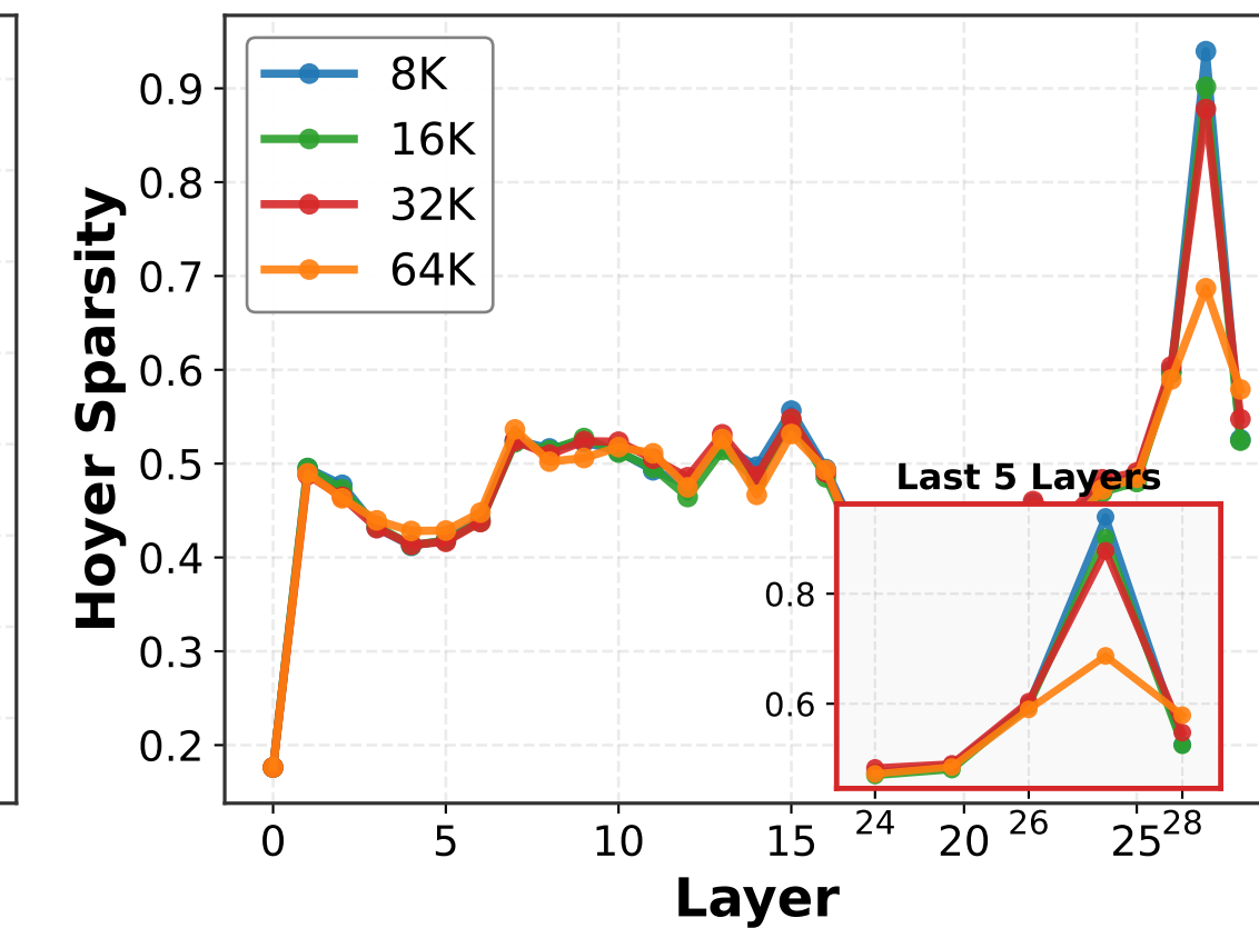
Hoyer Sparsity
