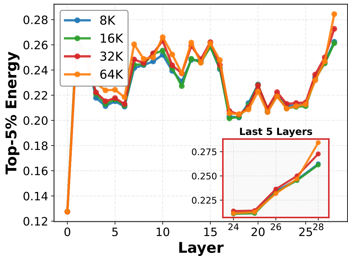
Top-5% Energy
