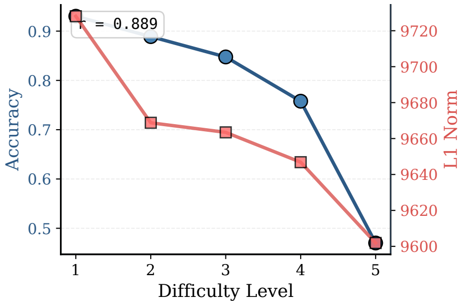
(a) Accuracy vs L1 Norm
