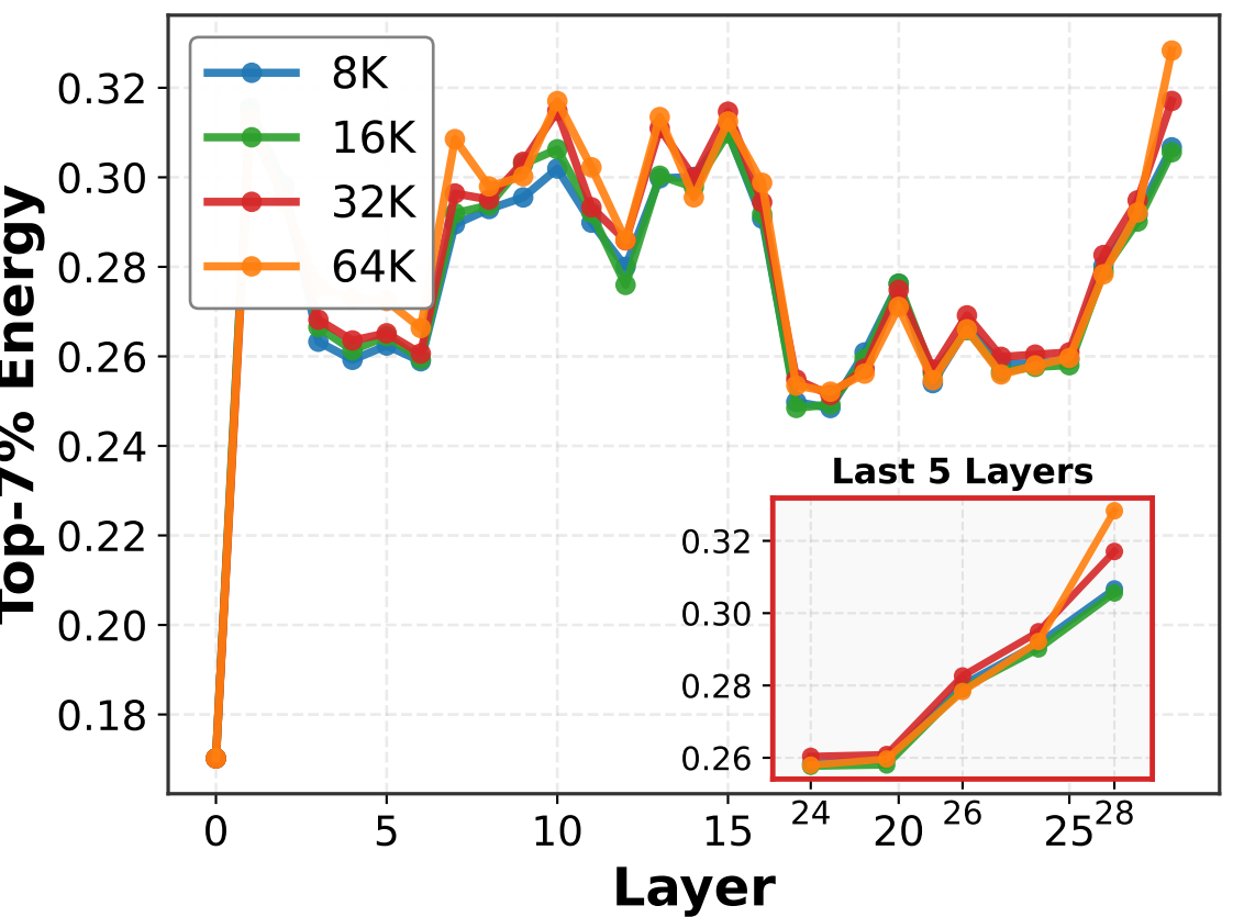
Top-7% Energy
