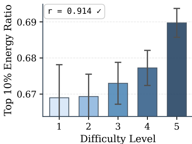
(b) Top 10% Energy Ratio - Qwen 2.5 7B
