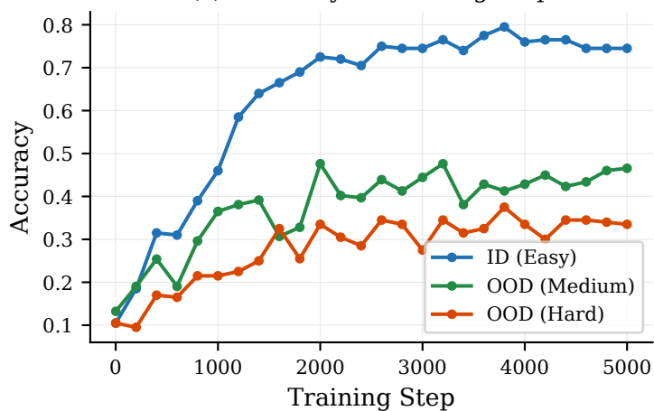
(c) Accuracy vs Training Step
