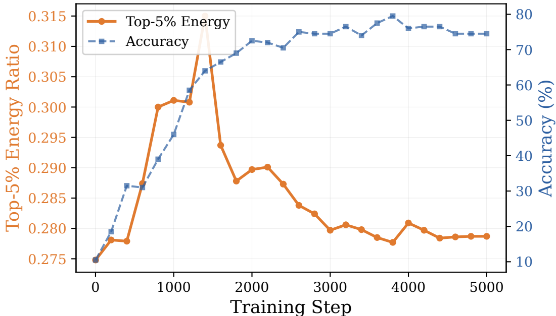
ID Sparsity Learning Dynamics (llama-32-32)
