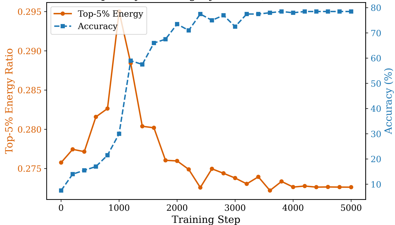
ID Sparsity Learning Dynamics (llama-16-16)
