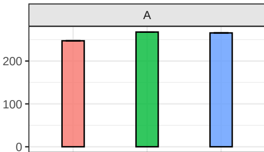
Average nROH per individual – 100 Mbps chr1 + simulation + dominant
