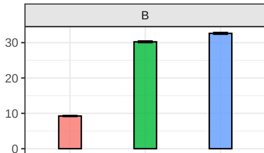
Average nROH per individual – whole chr1 + empirical
