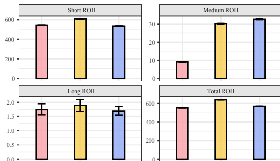
Empirical: Chr 1 (100 Mb)
