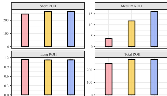
Simulated: Chr 1 (100 Mb, Dominant)
