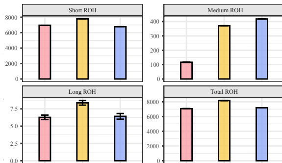
Empirical: Whole Chr 1
