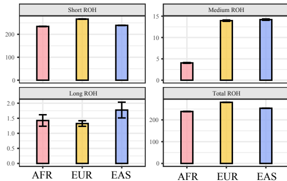
Empirical: Chr 1 (100 Mb)
