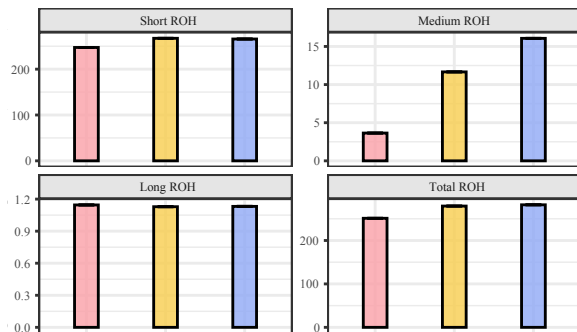
Simulated: Chr 1 (100 Mb, Additive)
