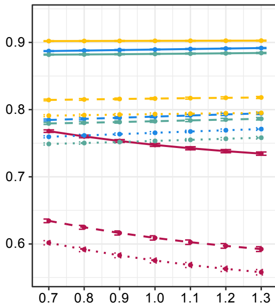
D Non-ROH
