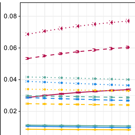
D Non-ROH
