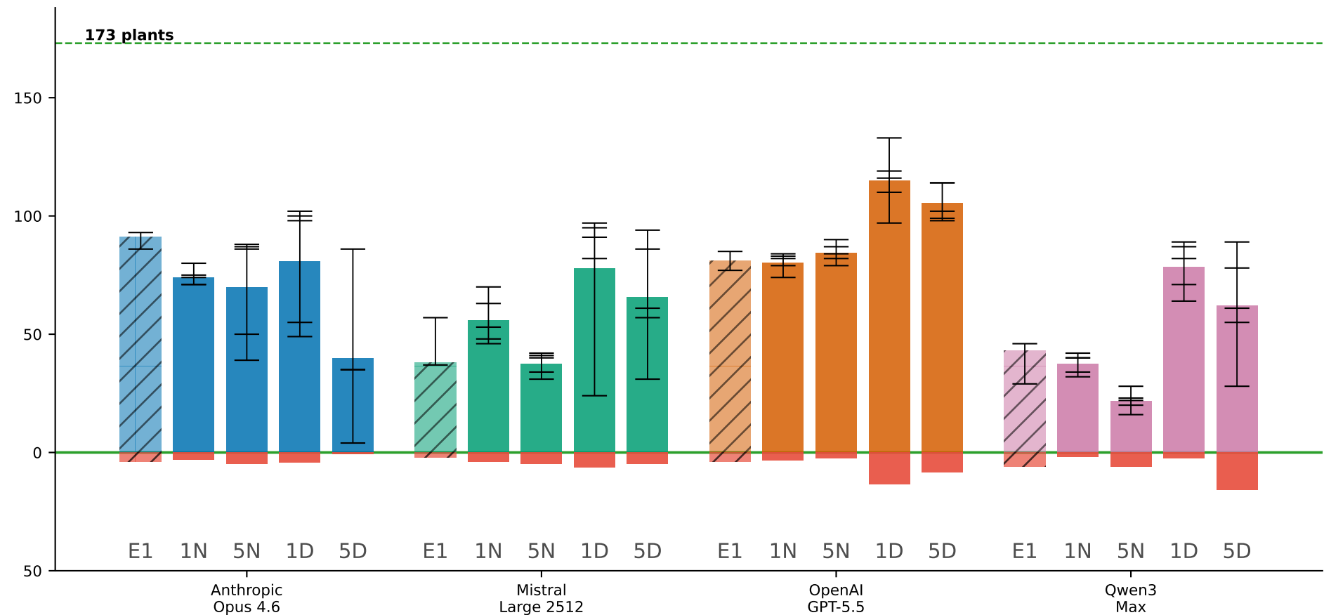
Number of assets identified (hatched = Exp 1 memory-only baseline; red = false positives)
