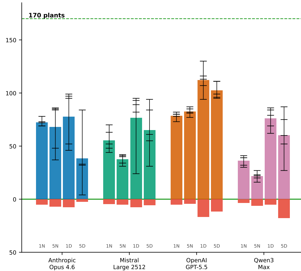
Number of assets identified (red are False Positives)
