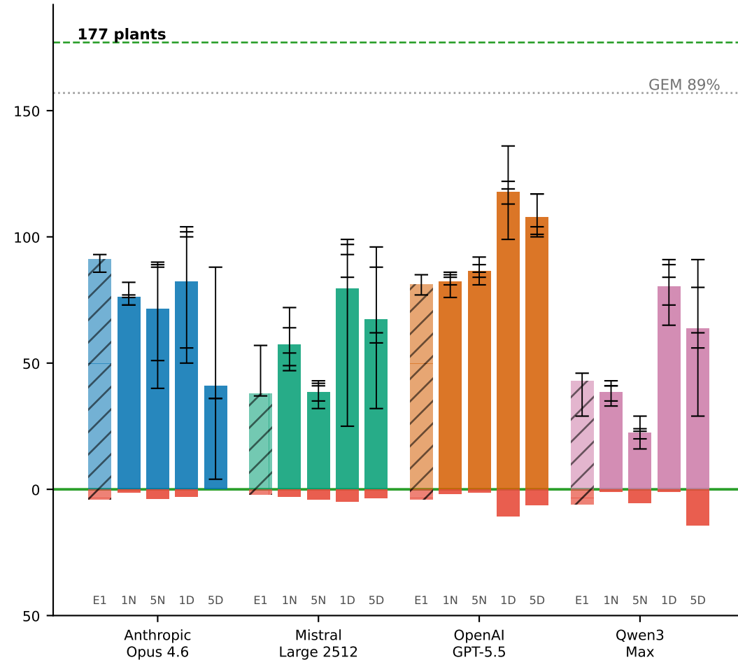
Number of assets identified (hatched = Exp 1 baseline; red = False Positives)
