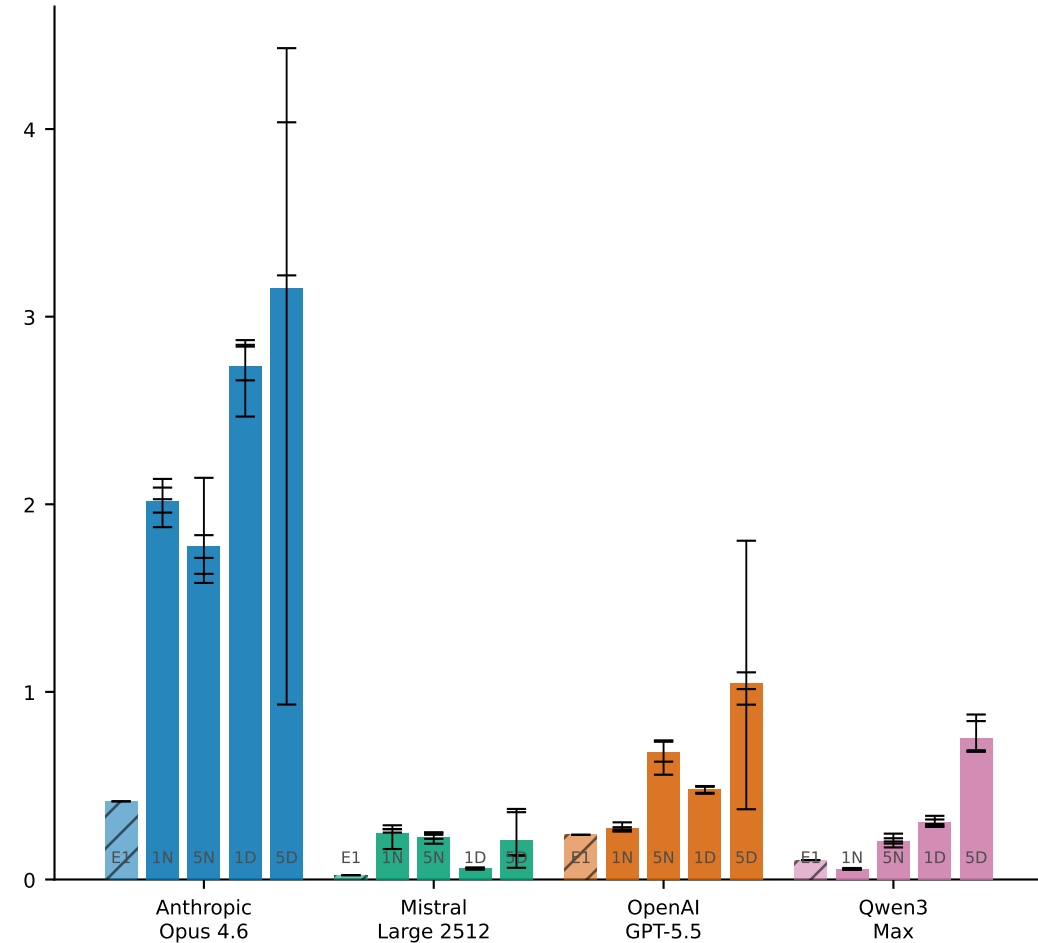
API cost per run, USD (hatched = Exp 1 baseline)
