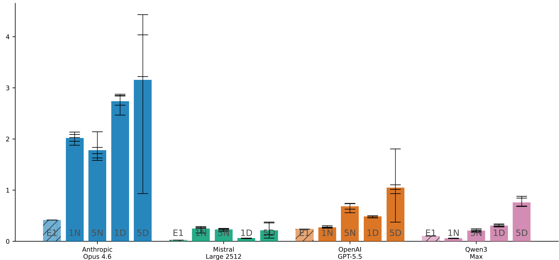
API cost per run, USD (hatched = Exp 1 memory-only baseline)
