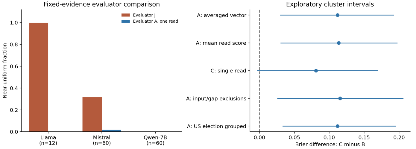
Fig. 1. Left: fixed-evidence near-uniform counts expressed as fractions (Table I). Right: exploratory Brier contrasts under alternative extraction and clustering choices (Table V). Bars on the left are observed fractions, not independent-agent estimates. Intervals on the right account for repeated campaigns within events; the grouped row additionally joins six US-election events.
