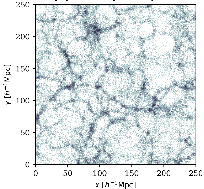
projected density, 15 h^{-1}\text{Mpc} slab
