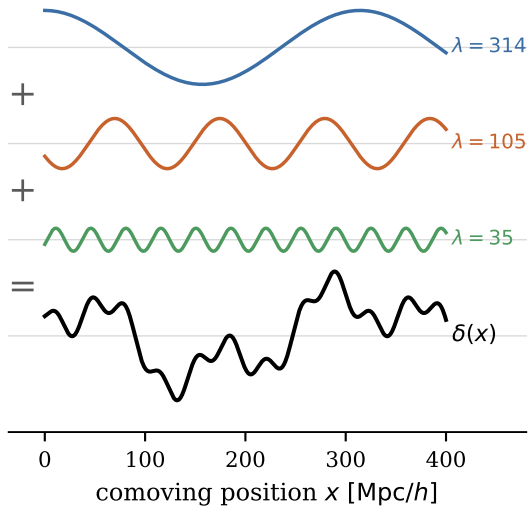
position space: a lumpy field
