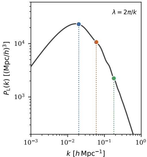
Fourier space: amplitude per mode
