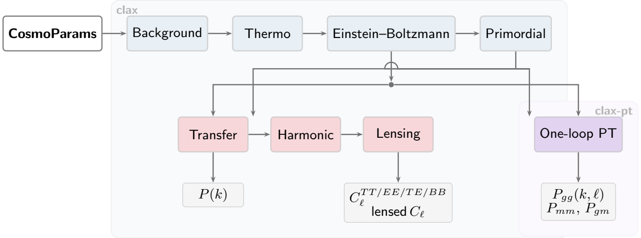
Figure 1. Pipeline architecture of CLAX and CLAX-PT. The shared backbone (top row) computes background cosmology, recombination, and the Einstein-Boltzmann perturbation hierarchy. Two branches produce CMB angular power spectra (left, via line-of-sight integration and lensing) and galaxy power spectrum multipoles (right, via one-loop EFT perturbation theory). Every module is independently validated against CLASS v3.3.4 (CLAX) or CLASS-PT (CLAX-PT) reference data. The entire pipeline is end-to-end differentiable: jax.grad propagates exact reverse-mode gradients from any output back to CosmoParams .
