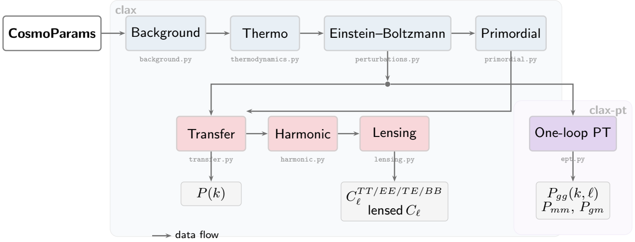
Figure 1. Pipeline architecture of CLAX and CLAX-PT. The shared backbone (top row) computes background cosmology, recombination, and the Einstein–Boltzmann perturbation hierarchy. Two branches produce CMB angular power spectra (left, via line-of-sight integration and lensing) and galaxy power spectrum multipoles (right, via one-loop EFT perturbation theory). Every module is independently validated against CLASS v3.3.4 (CLAX) or CLASS-PT (CLAX-PT) reference data. The entire pipeline is end-to-end differentiable: jax.grad propagates exact reverse-mode gradients from any output back to CosmoParams .
