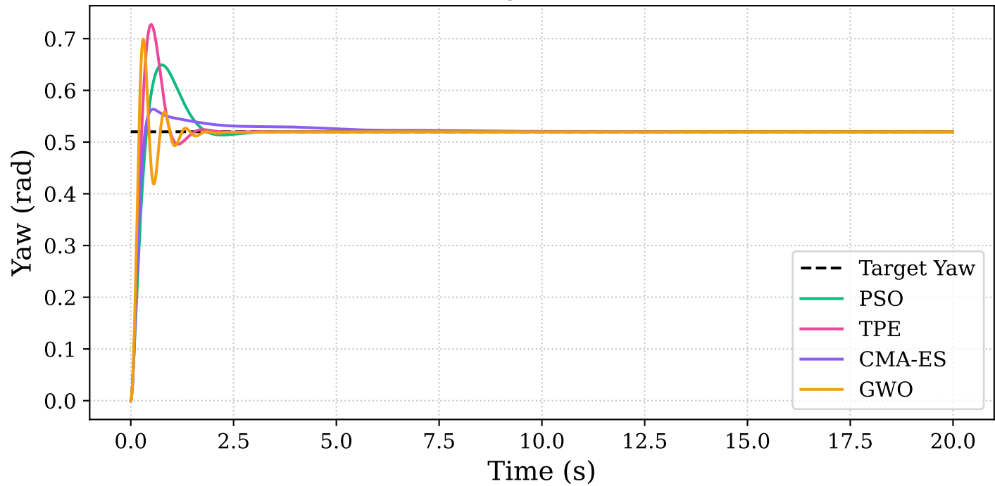
Yaw Angle Response
