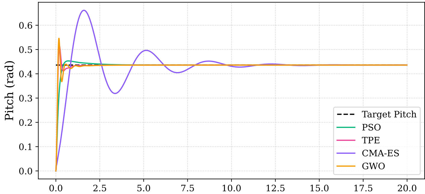
Pitch Angle Response
