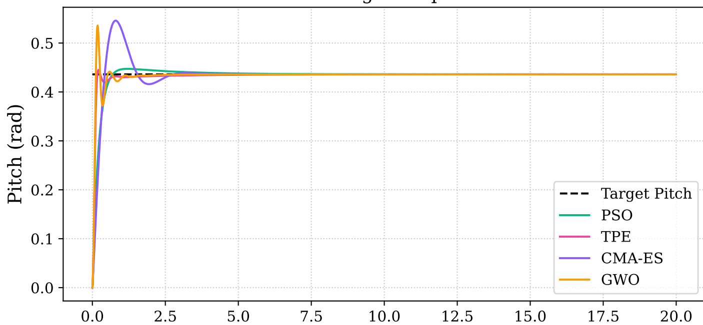
Pitch Angle Response
