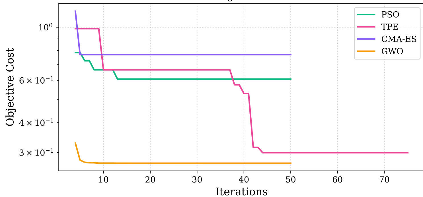
Convergence Curve
