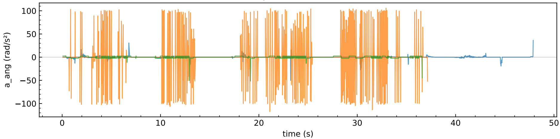
Angular acceleration
