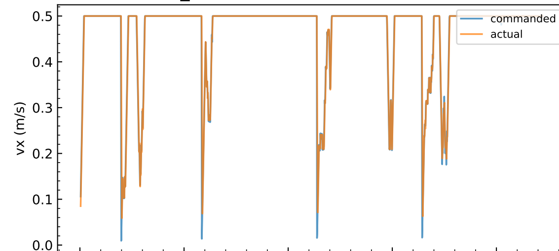
TD3_delta: commanded vs actual vx
