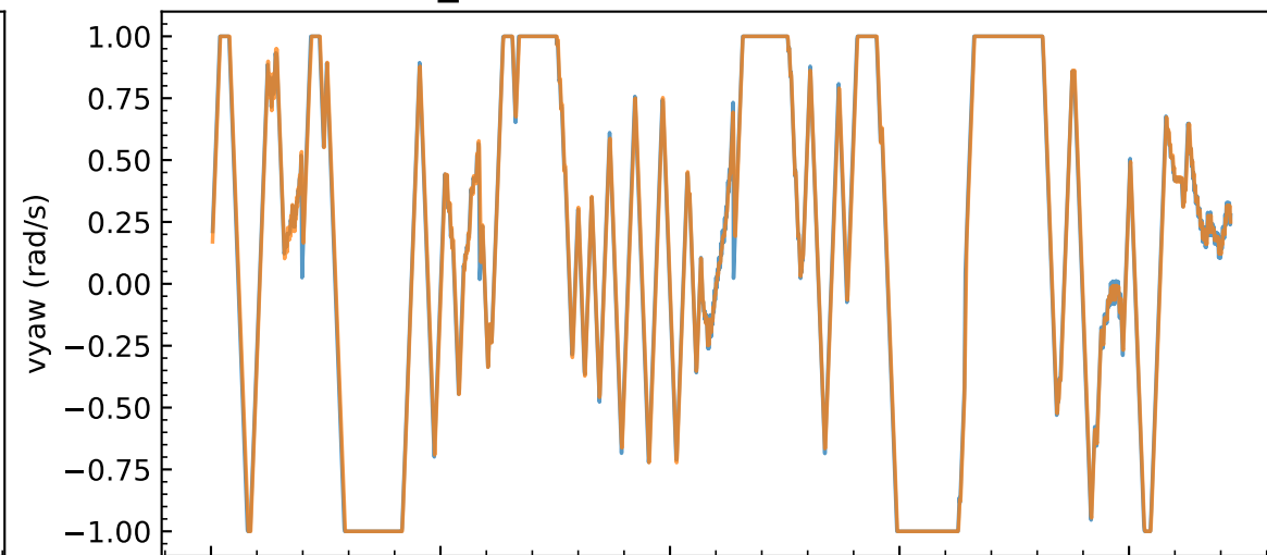
TD3_delta: commanded vs actual \omega
