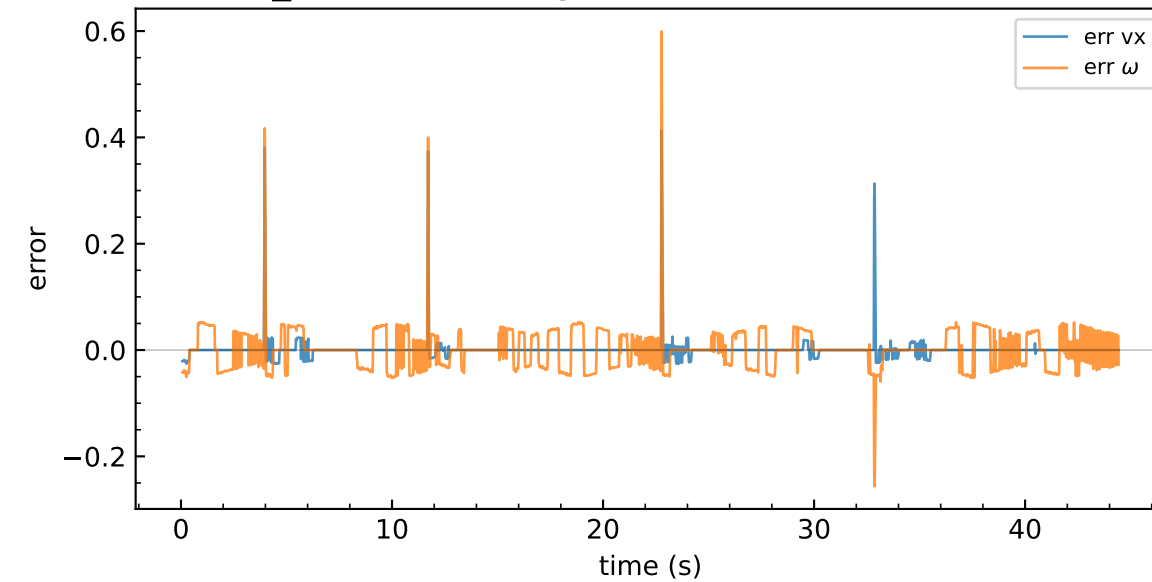
TD3_delta - tracking error (actual - commanded)
