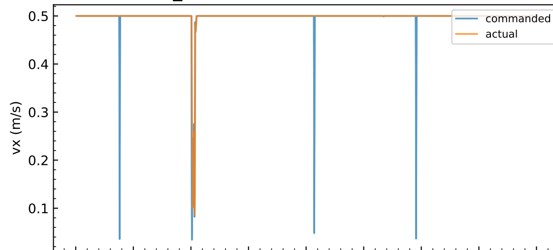
TD3_direct: commanded vs actual vx
