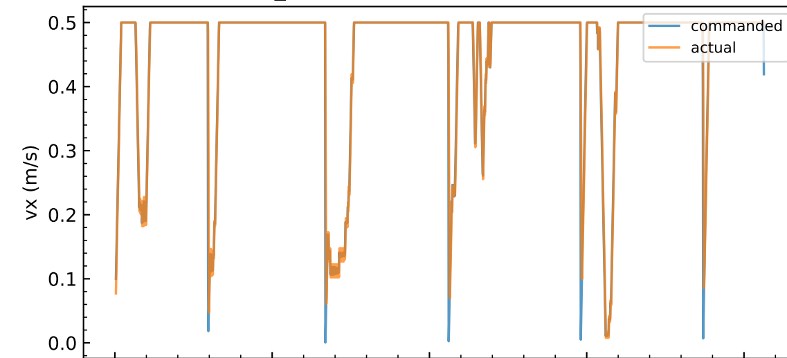
TD3_delta - vx: commanded vs actual
