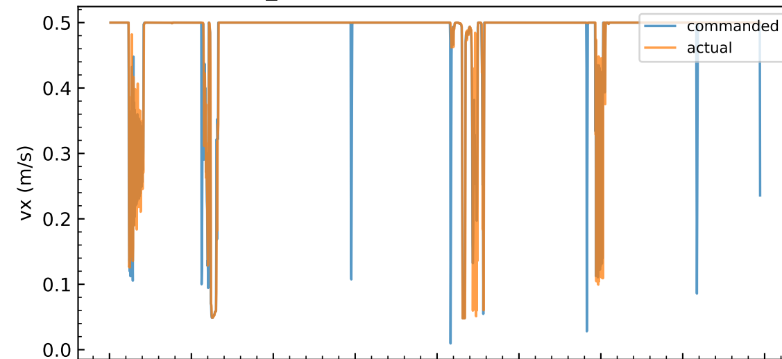
TD3_direct - vx: commanded vs actual
