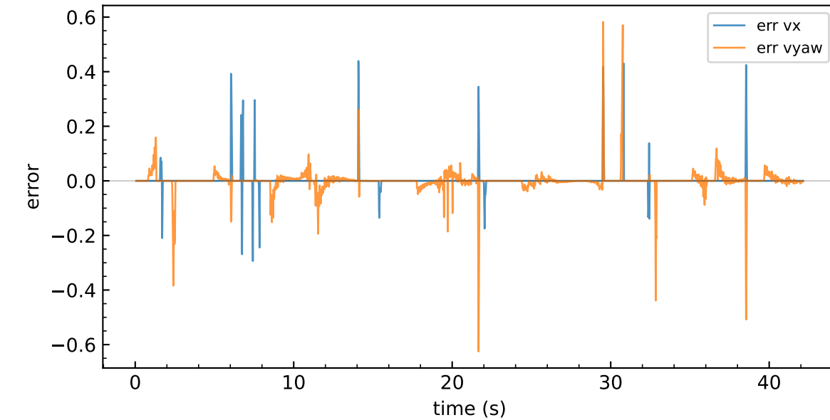
APF - tracking error (actual - commanded)
