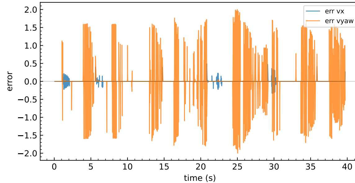
TD3_direct - tracking error (actual - commanded)
