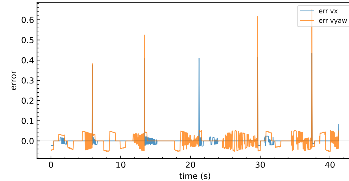
TD3_delta - tracking error (actual - commanded)
