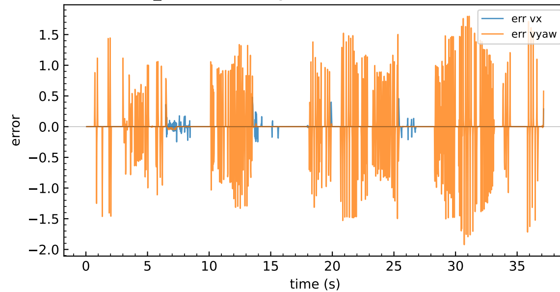
TD3_direct - tracking error (actual - commanded)
