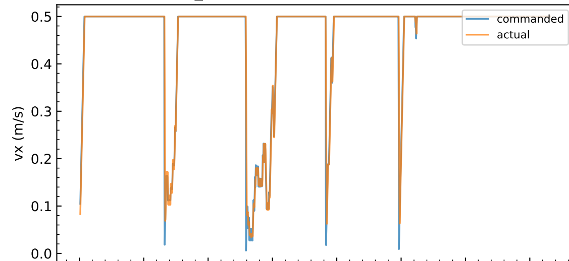
TD3_delta - vx: commanded vs actual
