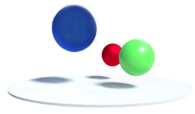
bouncingballs
