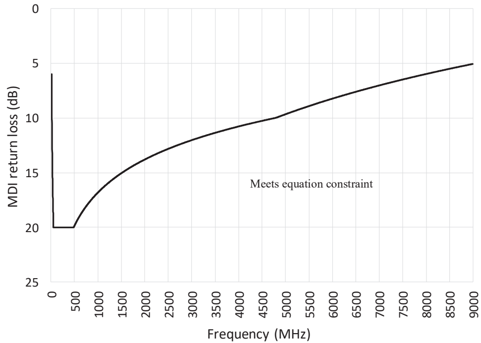
Figure 165-38—MDI return loss calculated limit in Equation (165-42)
