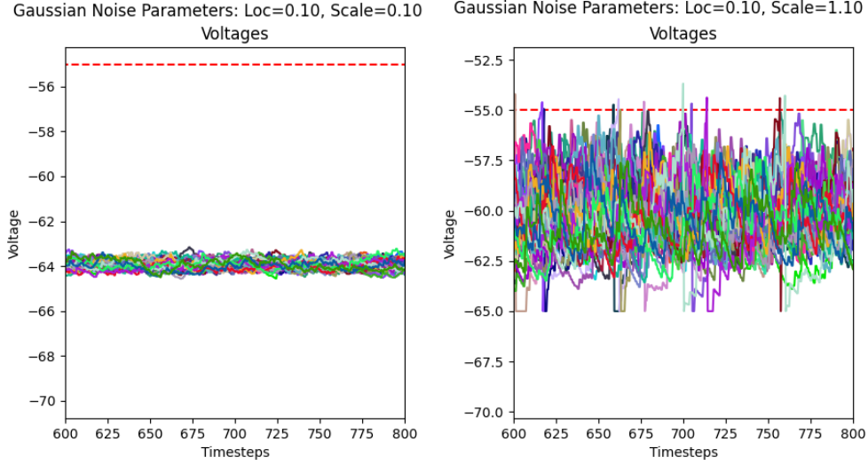
Figure 2: Voltage Recordings with Zero Interconnectivity in the 600-800ms Window
