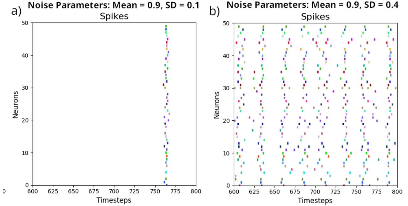
Figure 4: Visual Comparison of Spike Pattern Length in a Network with 20 mV Lateral Weights
