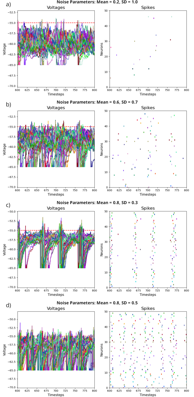
Figure 3: Spike Behavior in Different Noise Conditions and Corresponding Voltages for 20 mV Connectivity Weights
