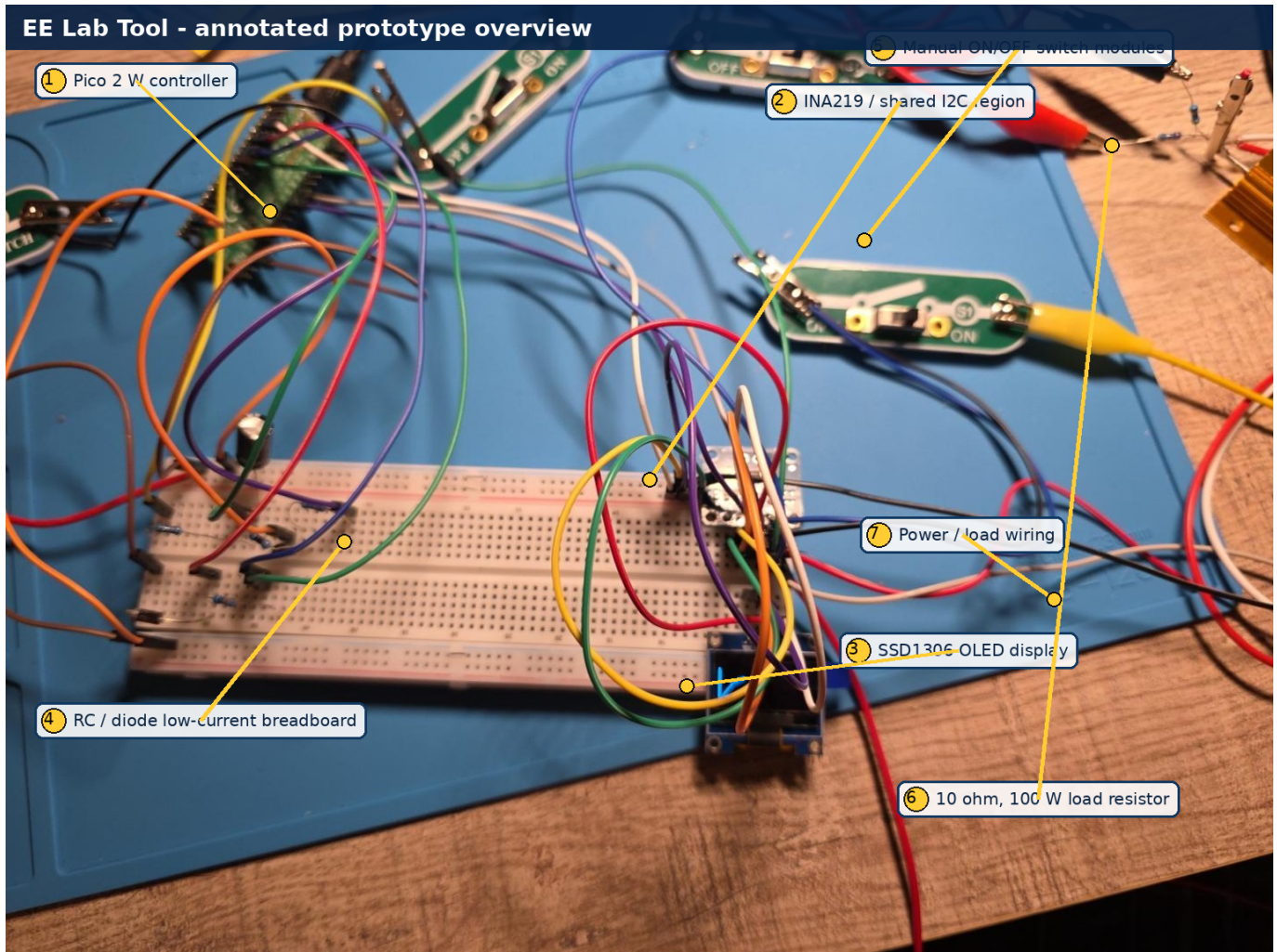
Real sanitized prototype photograph with subsystem callouts.
