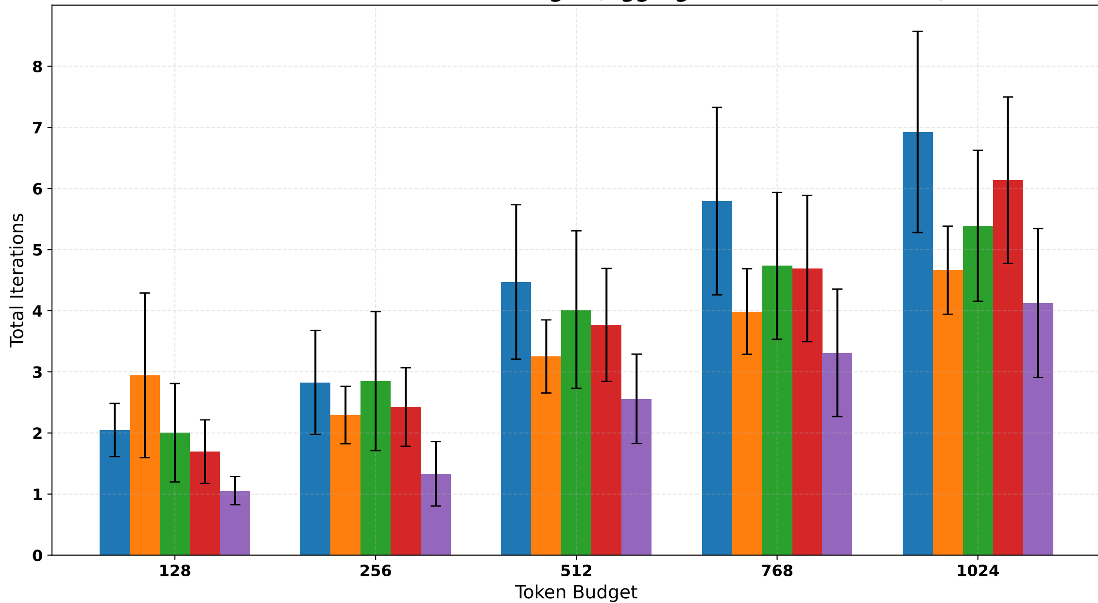
PCCR Iterations vs Token Budget (Aggregated Across Datasets)
