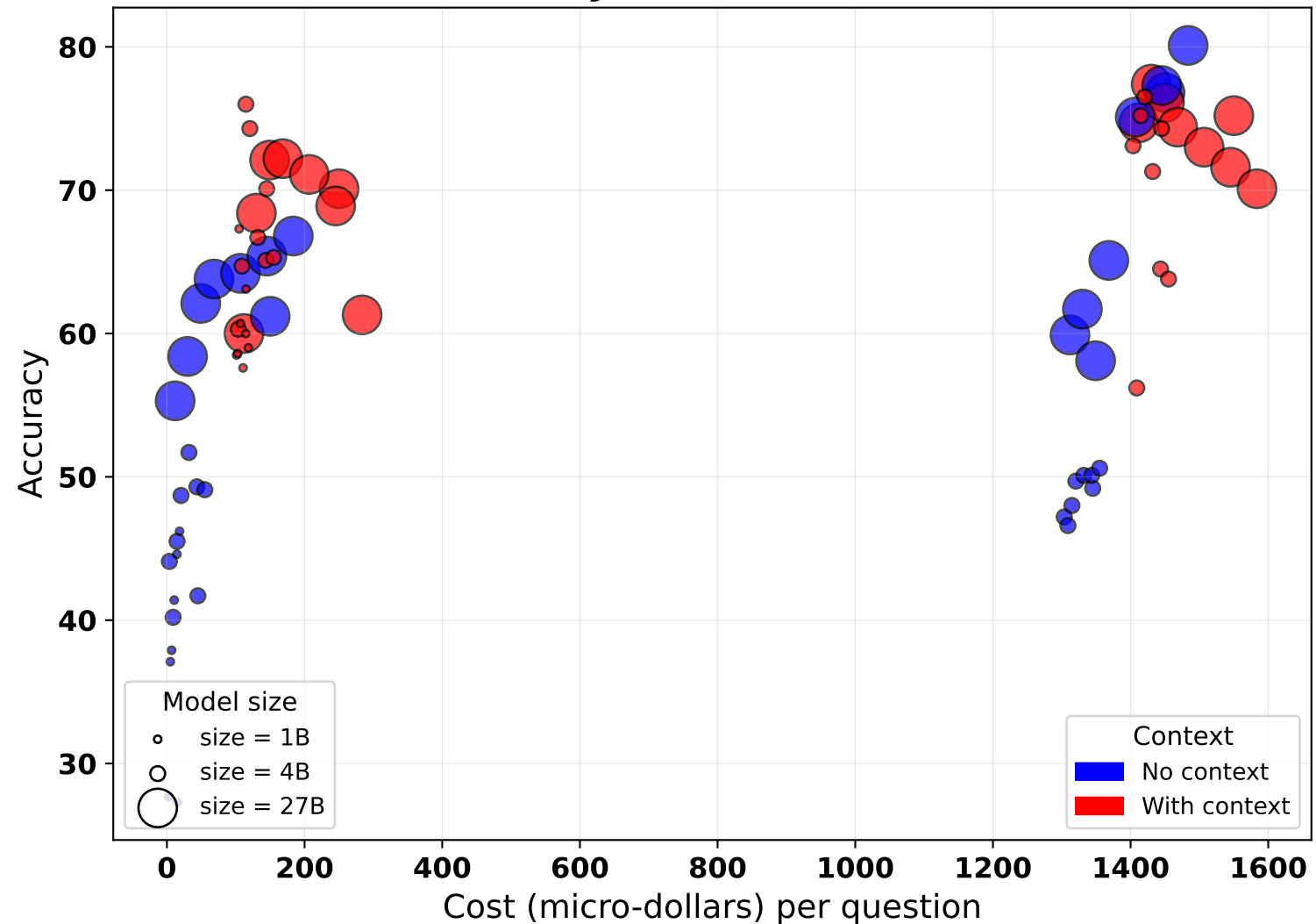
Accuracy vs Estimated Cost
