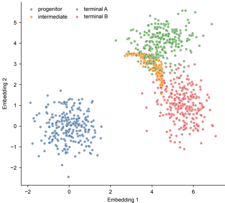
Single-cell differentiation manifold
