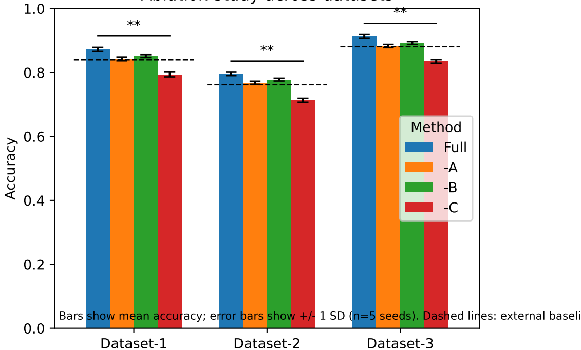
Ablation study across datasets
