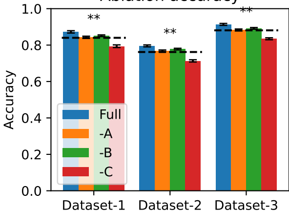
Ablation accuracy
