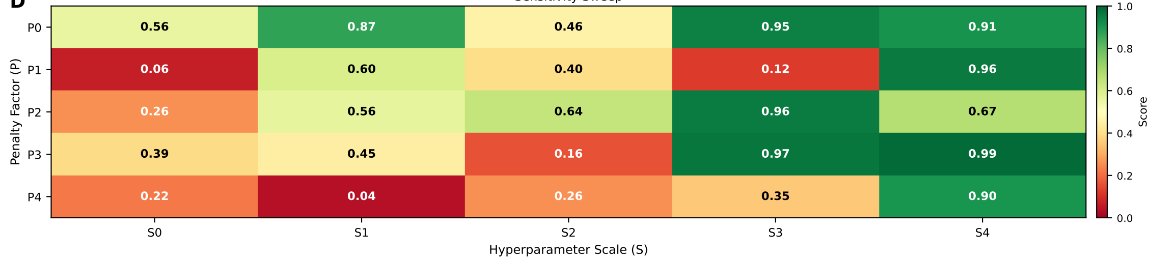
Sensitivity Sweep
