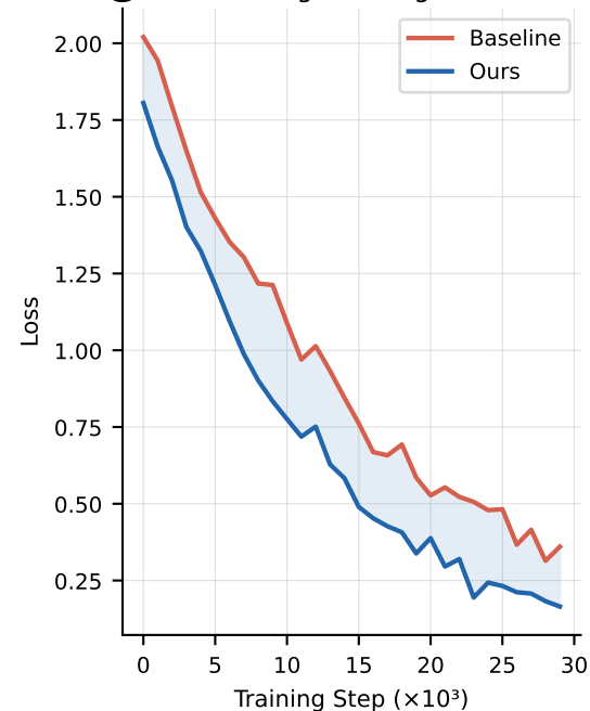
Training Convergence
