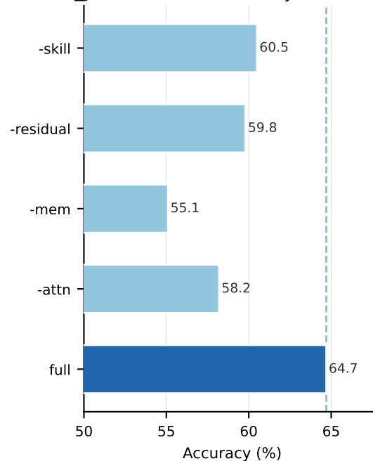
Ablation Study
