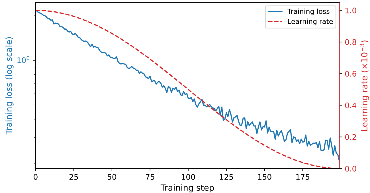
Training dynamics: loss and cosine LR schedule
