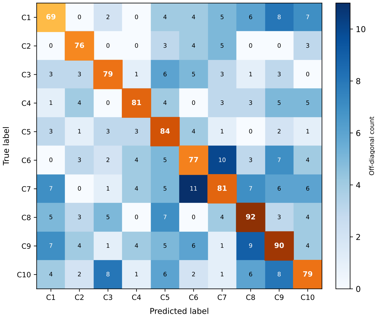
Confusion Matrix (10 classes)
