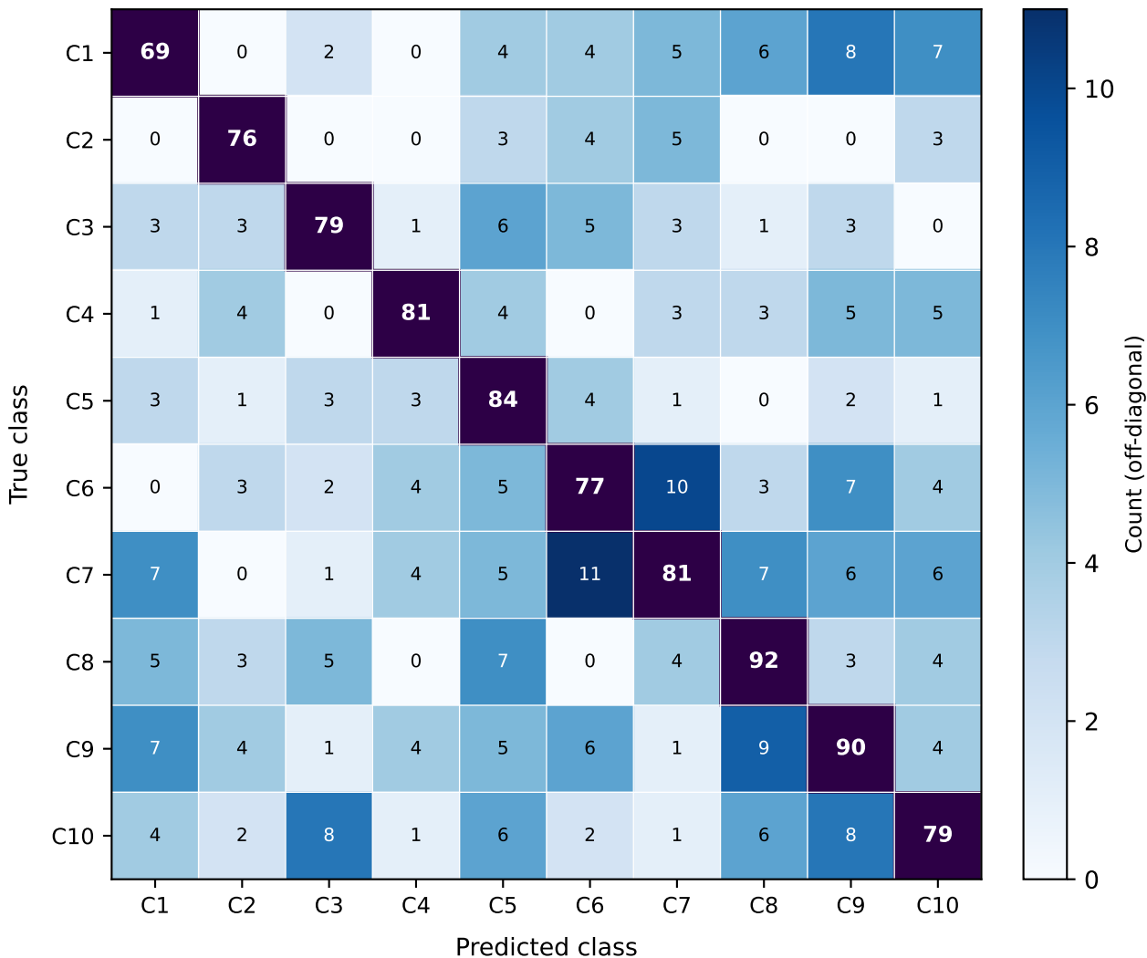
Confusion matrix (counts)
