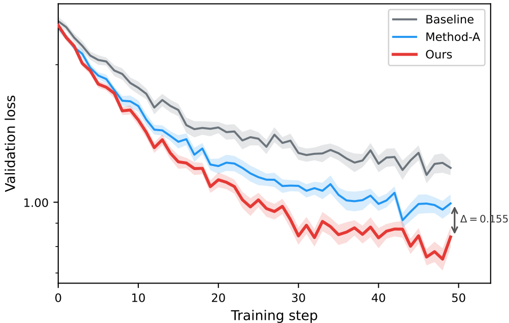
Validation Loss over Training (95% CI, n = 5 )
