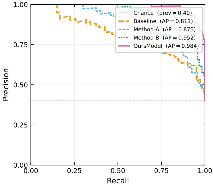
Precision-Recall curve
