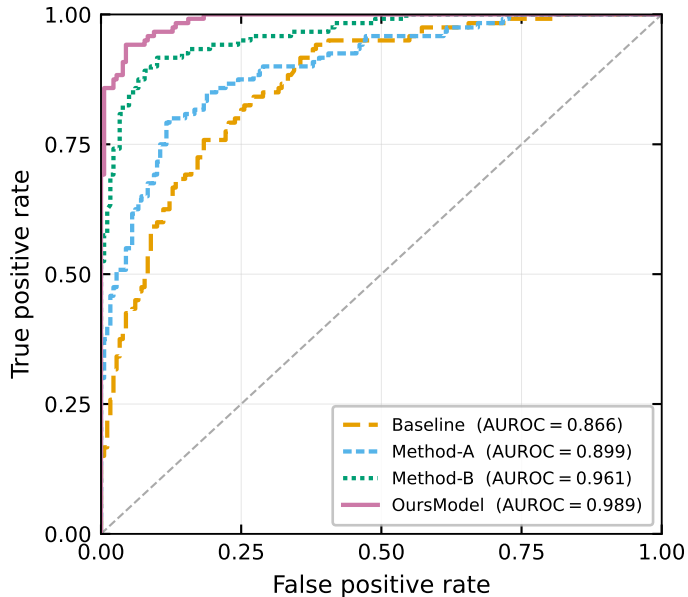
ROC curve
