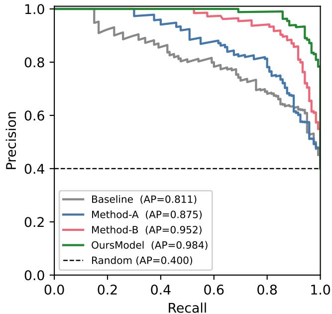
Precision-Recall Curve
