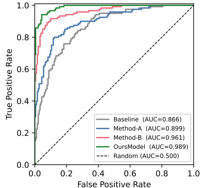
ROC Curve
