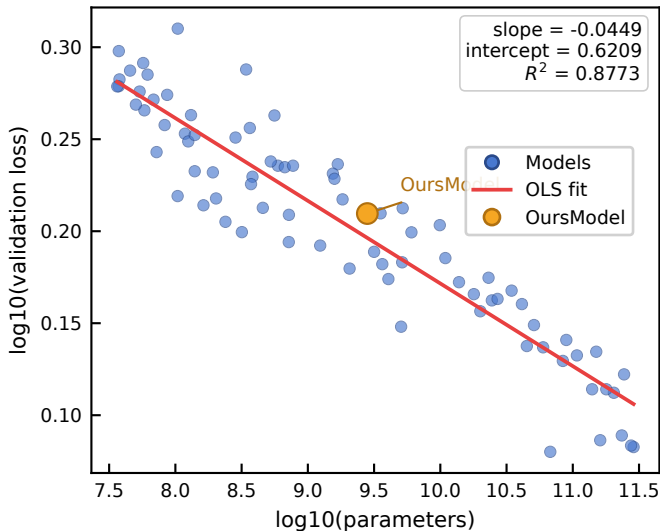
Neural Scaling Law: Parameters vs. Validation Loss
