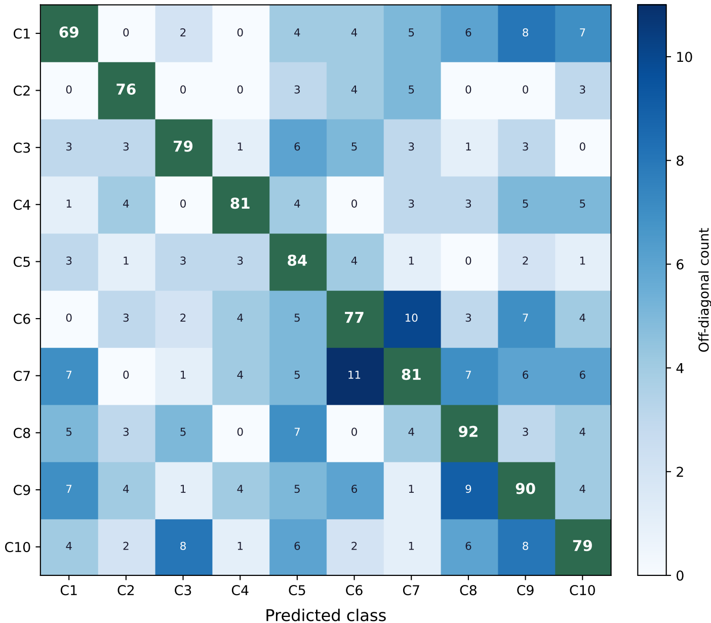
10-Class Confusion Matrix
