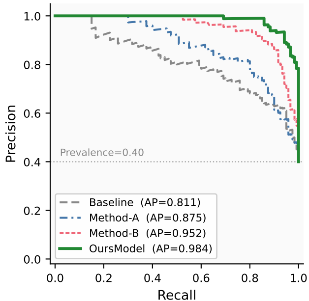
Precision-Recall Curve
