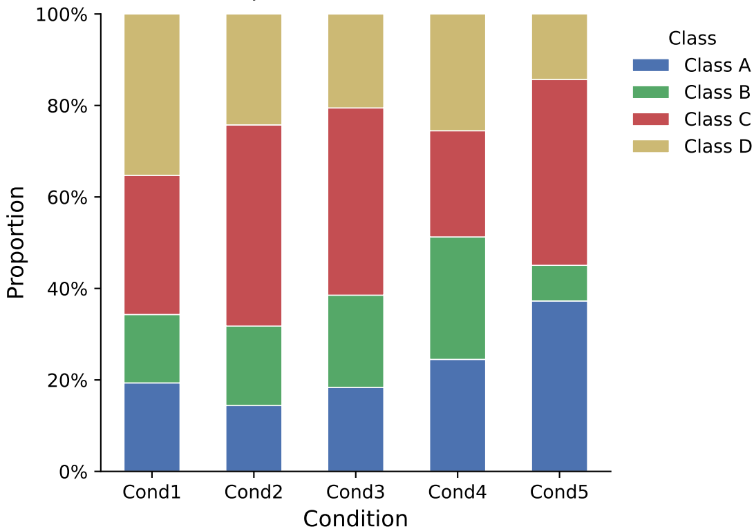
Class Proportions Across Conditions
