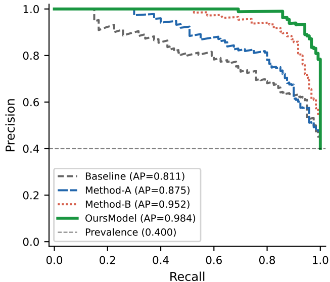
Precision-Recall Curve
