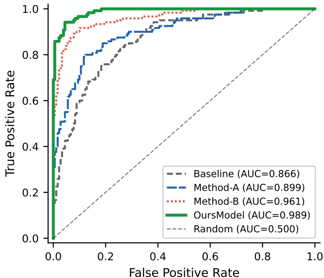
ROC Curve
