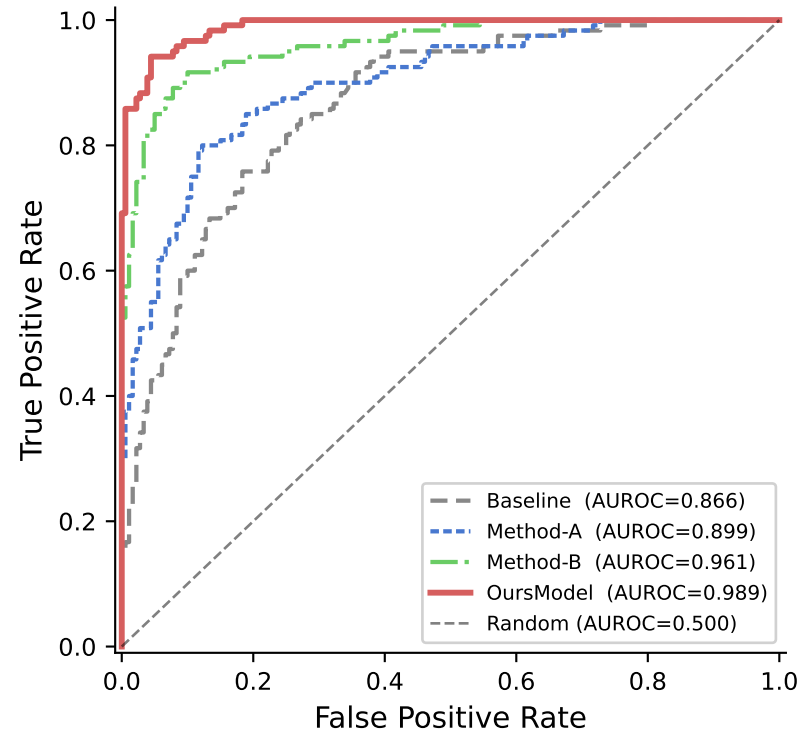
ROC Curve
