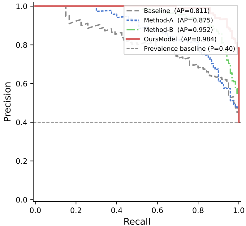
Precision-Recall Curve
