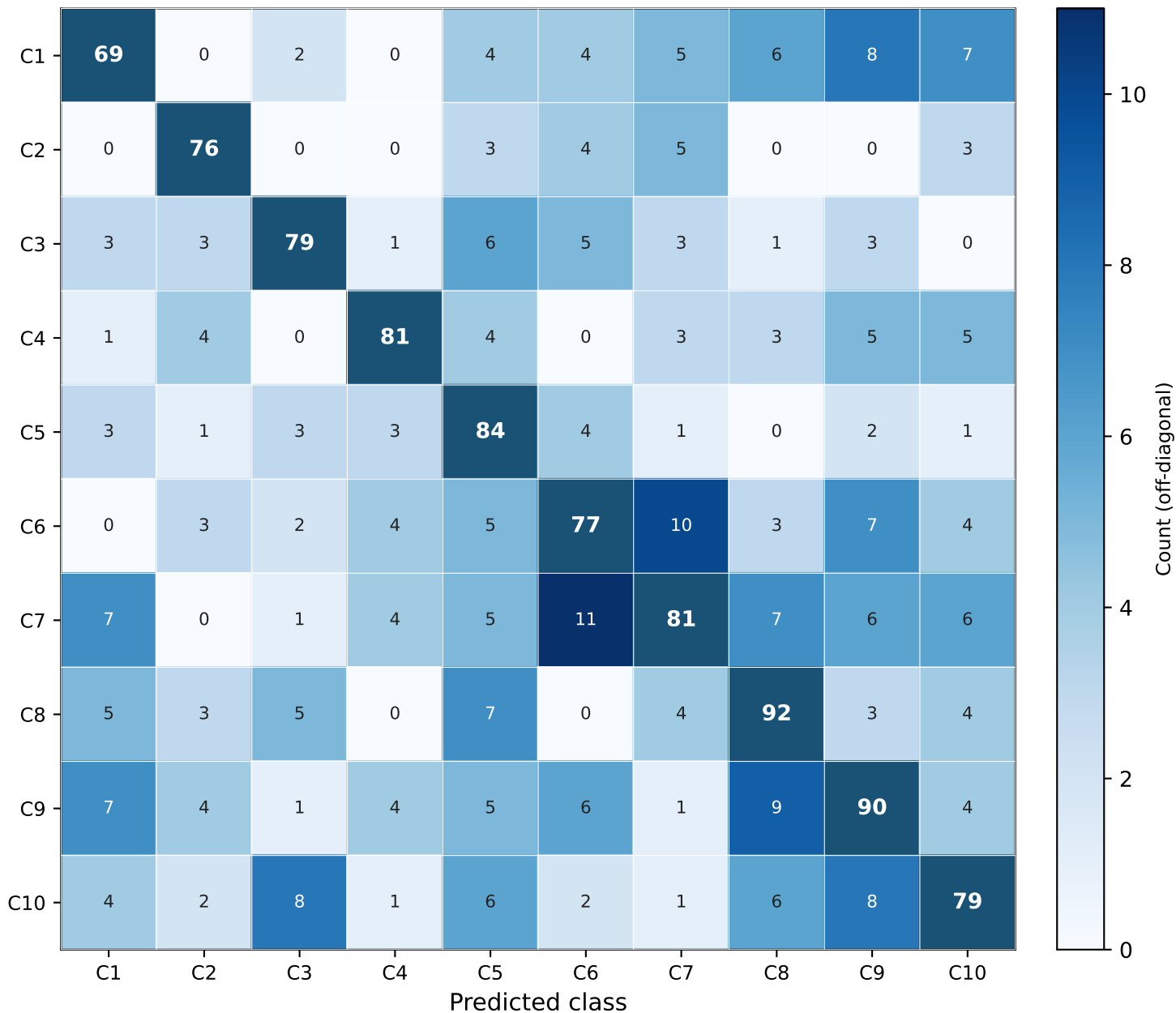
10×10 Confusion Matrix
