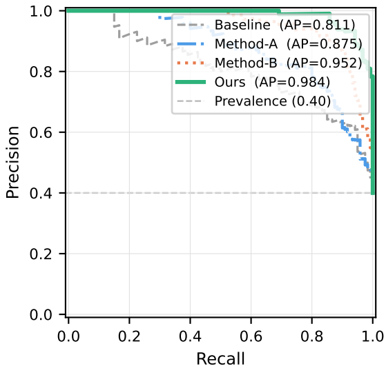
Precision-Recall Curve
